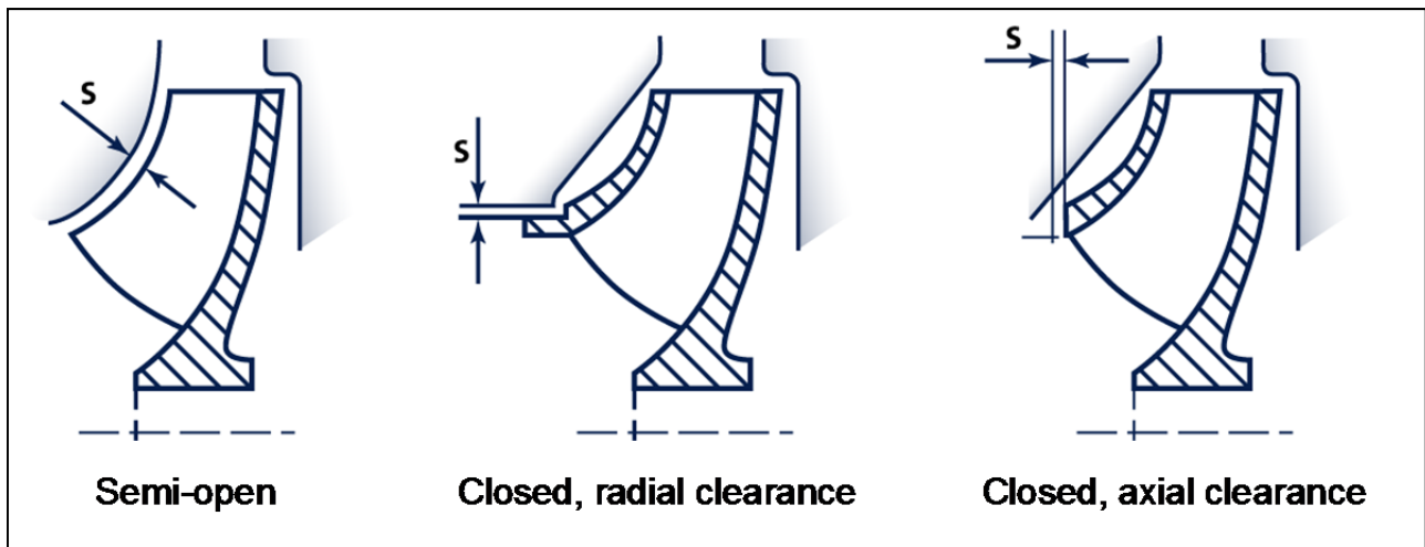
Wear of impeller clearances with different impeller designs
